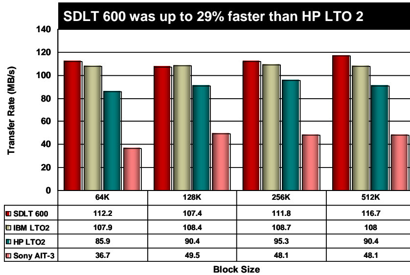
Figure 2. READ Transfer Rate Test Results w/Compression ON
