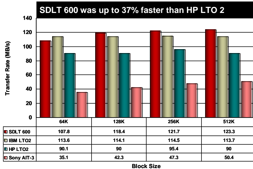
Figure 1. WRITE Transfer Rate (MB/s) Test Results w/Compression ON
